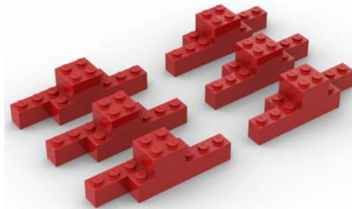
Rocks
